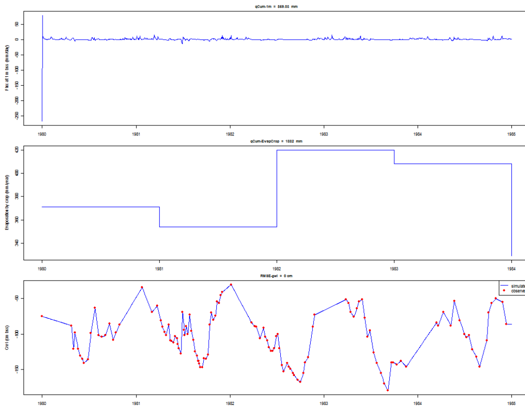
Figuur 12: GwlMeasuredasbottomBC(Ruurlo)
