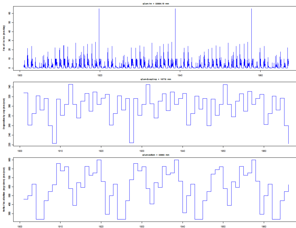
Figuur 26: PearlFocus3(Port-m)
