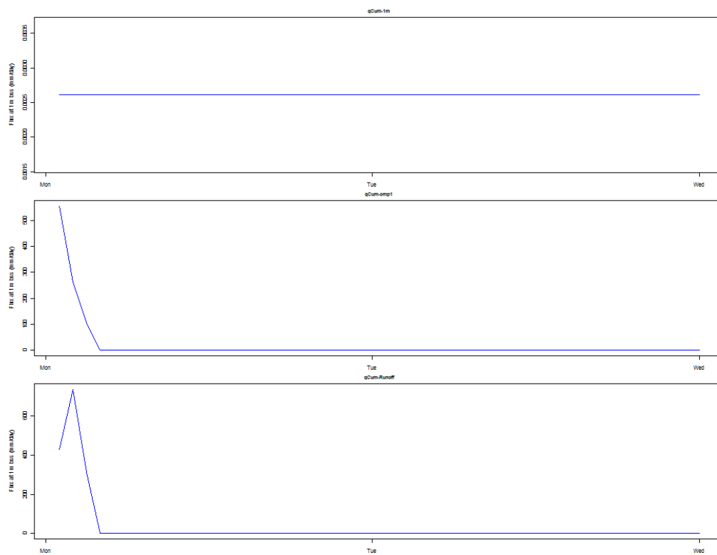
Figuur 15: InfiltrationRunoff(VanDamFeddes2000)
