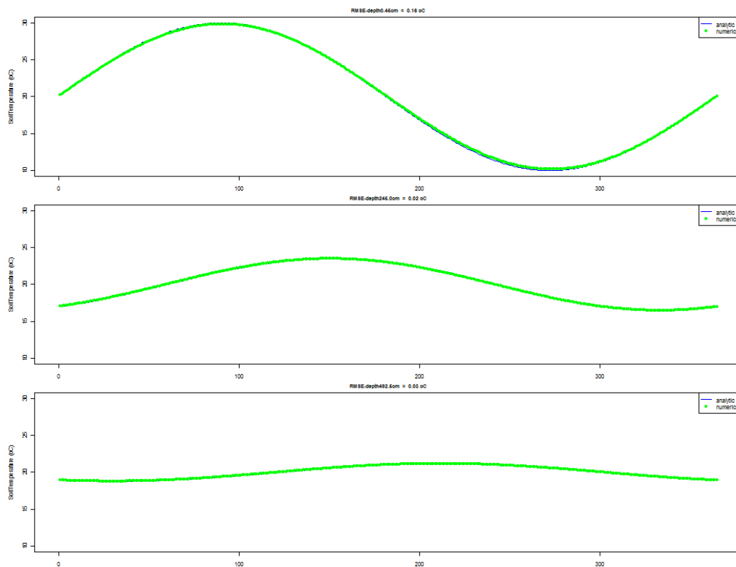
Figur 2: AnalyticSoilTemperature
