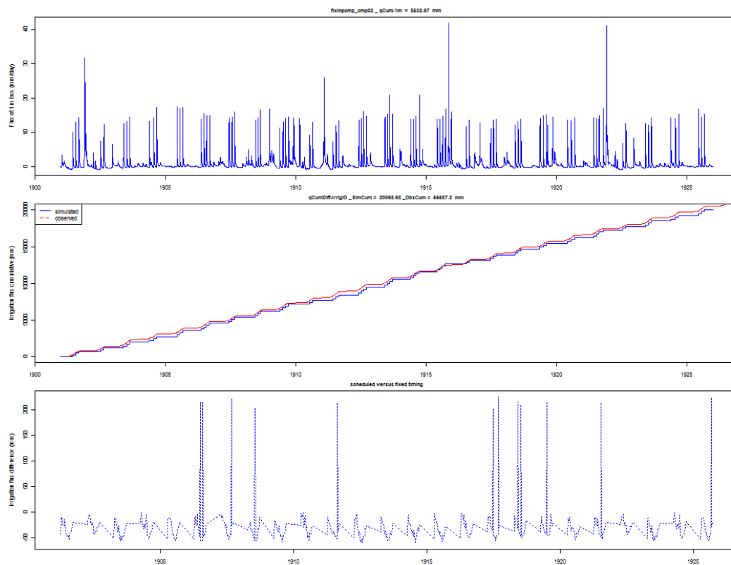
Figuur 18: IrrigationScheduledFixedTiming(Sevilla)
