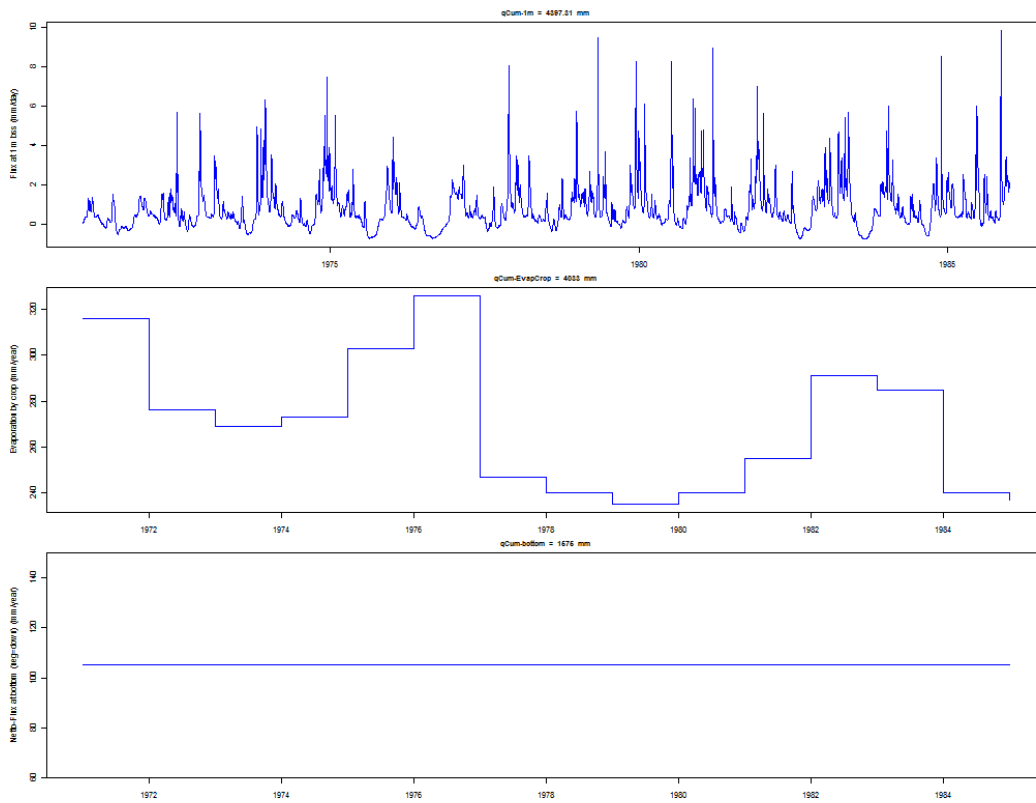
Figur 9: DrainageExtended(STONE2uc6)
