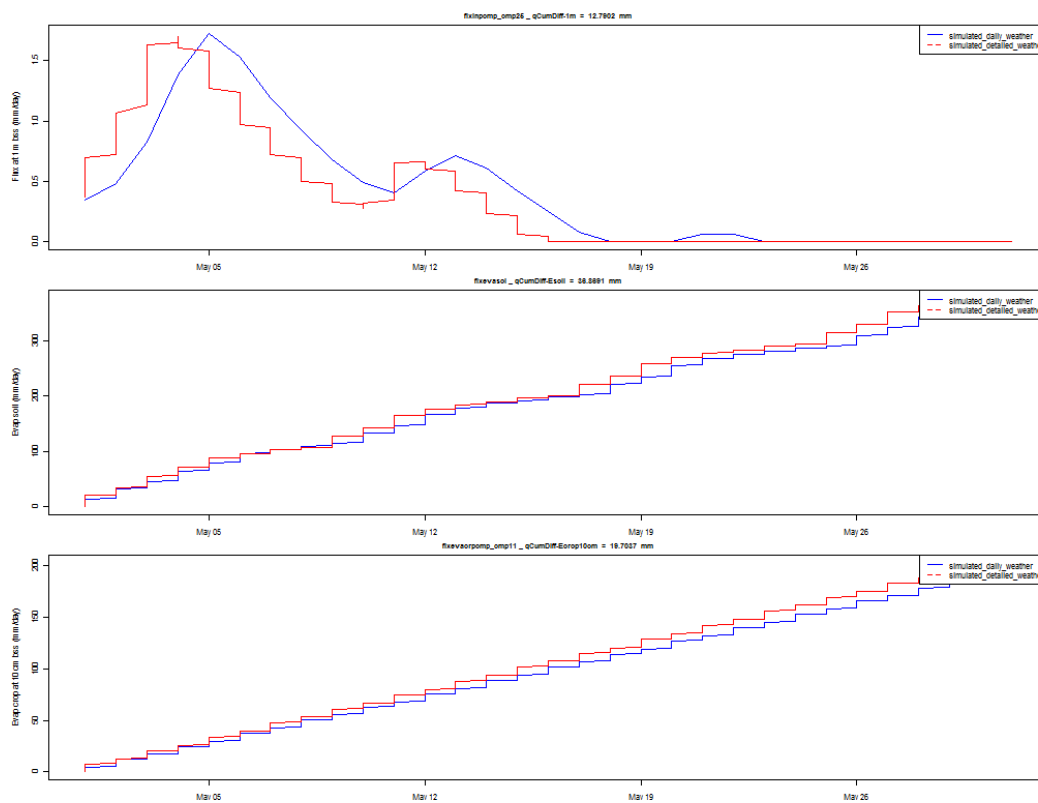
Figure 21: MeteoDetailedInOut(Hupsel)
